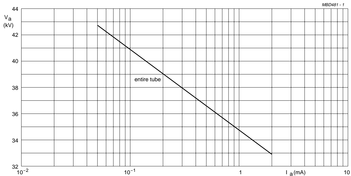
Fig.16 0.5 mR/h iso-exposure-rate limit curve.
