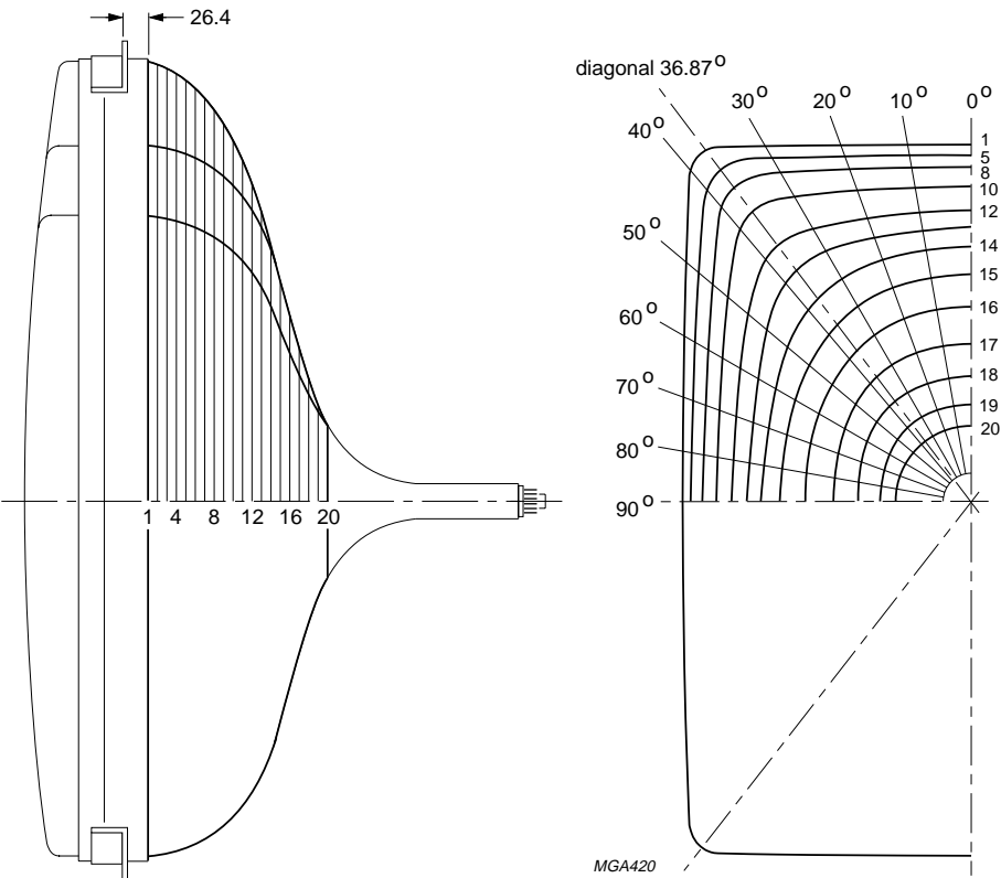
Fig.12 Maximum cone contour.
